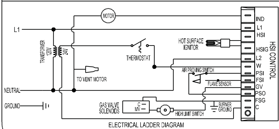
ELECTRICAL CONNECTION DIAGRAM
